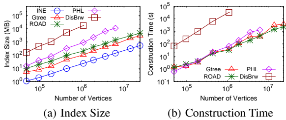
Figure 8: Effect of Road Network Size |V|
