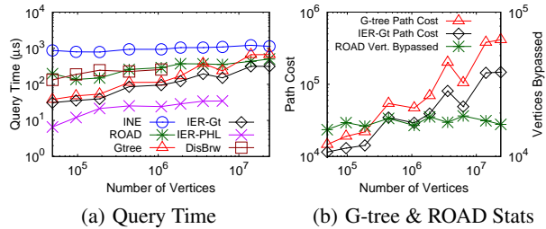
Figure 9: Effect of Road Network Size |V| ( d=0.001, k=10 )
